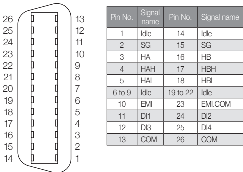
FX5-40SSC-S
