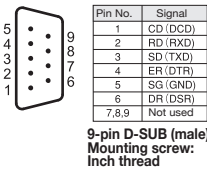
FX5-232ADP
