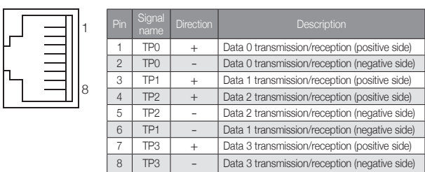
FX5-CCLIEF
